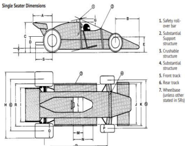
Single Seater Dimensions
