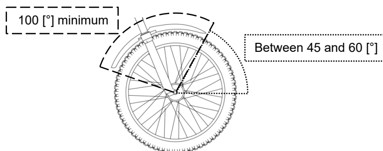
Figure 10 : Front mudguard position
