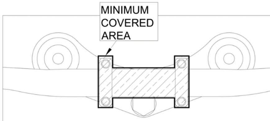
Figure 2 : Handlebar covering
