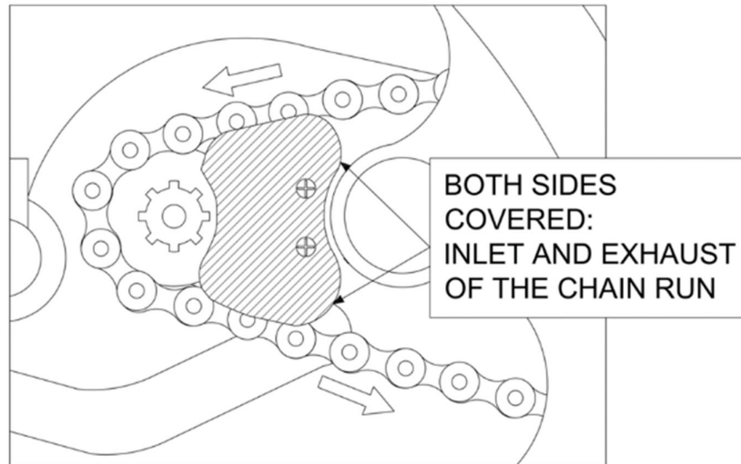
Figure 4 : Front sprocket protection
