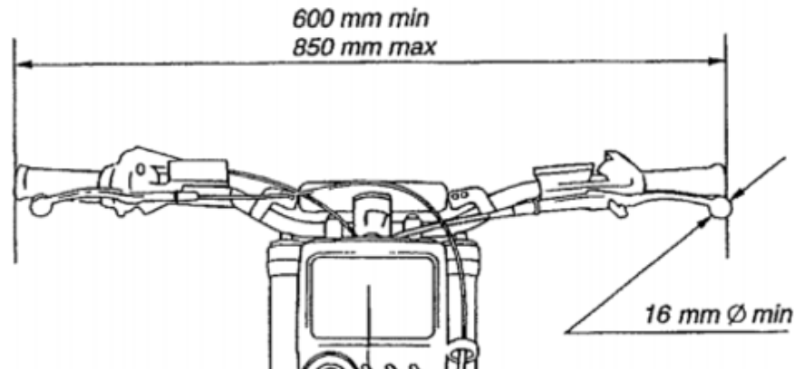
Figure 1 : Handlebar length
