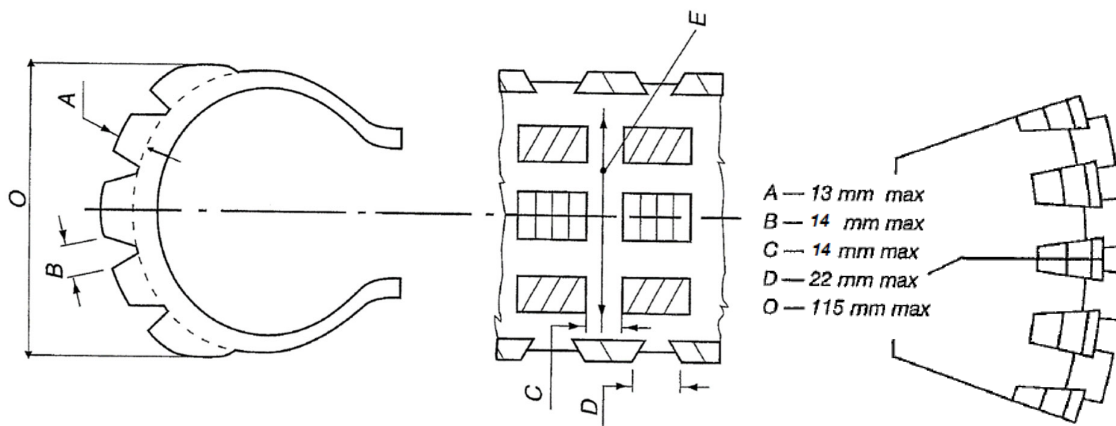
Figure 3 : Tyre dimensions
